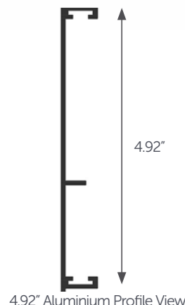
4.92" Aluminium Profile View
