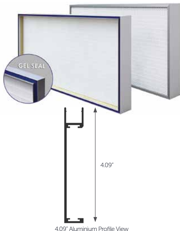
4.09" Aluminium Profile View
